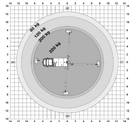
Working envelope
