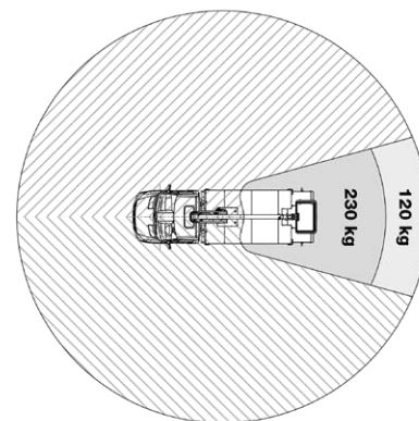
Turret/knuckle tail swing and outriggers within the mirrors
