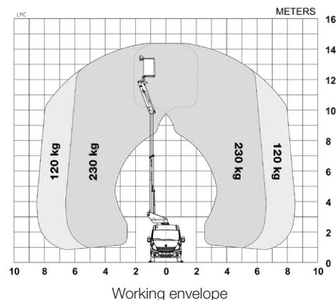
Working envelope
